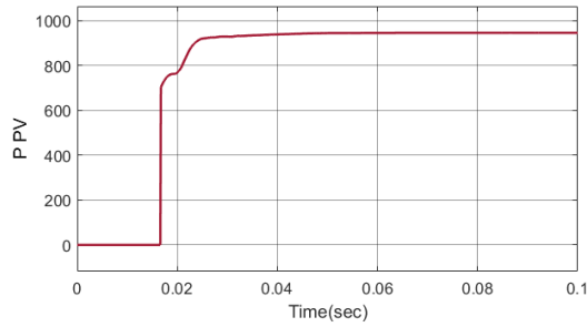
Figure 7. PV power and time characteristics
