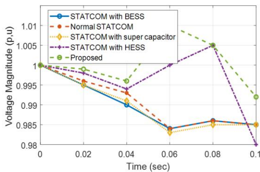
Figure 11. Comparison of proposed method with BESS, STATCOM, super capacitor, and HESS
