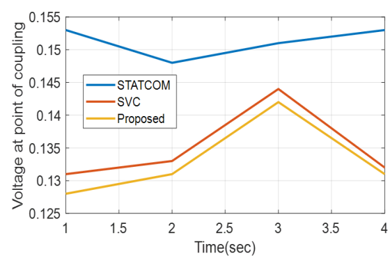
Figure 14. Comparison of proposed method with STATCOM and SVC (voltage at point of coupling vs time)
