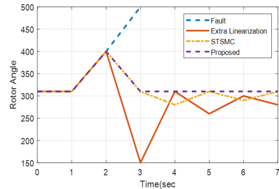
Figure 16. Comparison of proposed method with fault, extra linearization, and STSMC
