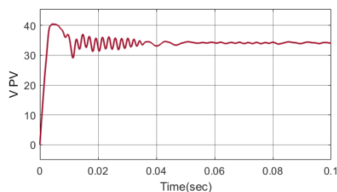
Figure 5. PV voltage and time characteristics
