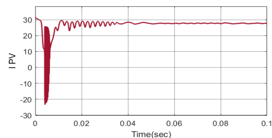
Figure 6. PV current and time characteristics
