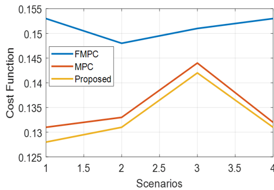
Figure 13. Comparison of proposed method with FMPC and MPC cost function vs scenarios (cost function vs scenarios)
