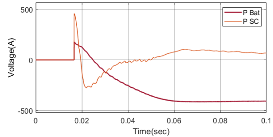
Figure 10. Voltage vs time characteristics of battery and super capacitor
