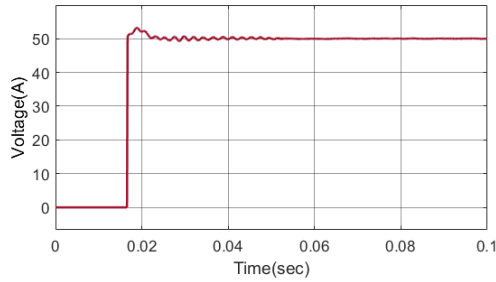
Figure 9. Voltage vs time characteristics (transient stability improvement)
