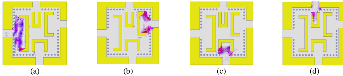
Figure 4. Resonating pattern (Magnetic field distribution) with “U”-shaped slot (a) port 1 ON, (b) port 2 ON, (c) port 3 ON, and (d) port 4 ON
