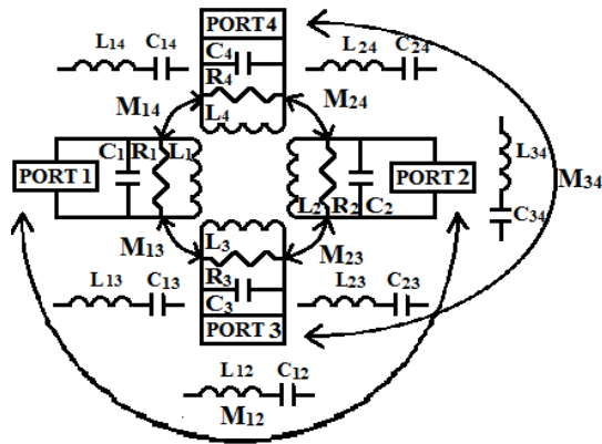
Figure 8. The equivalent circuit model of the proposed self-quadplexing slot antenna
