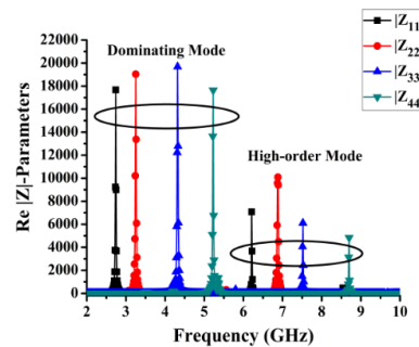
Figure 2. |Z| -parameters of the proposed SIW cavity
