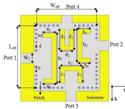
Figure 1. Geometry and top view of the proposed self-quadplexing antenna
