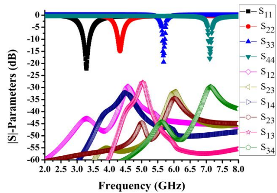
Figure 9. The simulated value of |S|-parameters of the proposed antenna by ADS software
