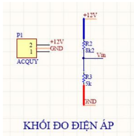
Figure 5. Circuit diagram of voltage measurement circuit
