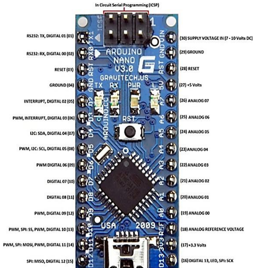
Figure 3. Arduino Nano board image
