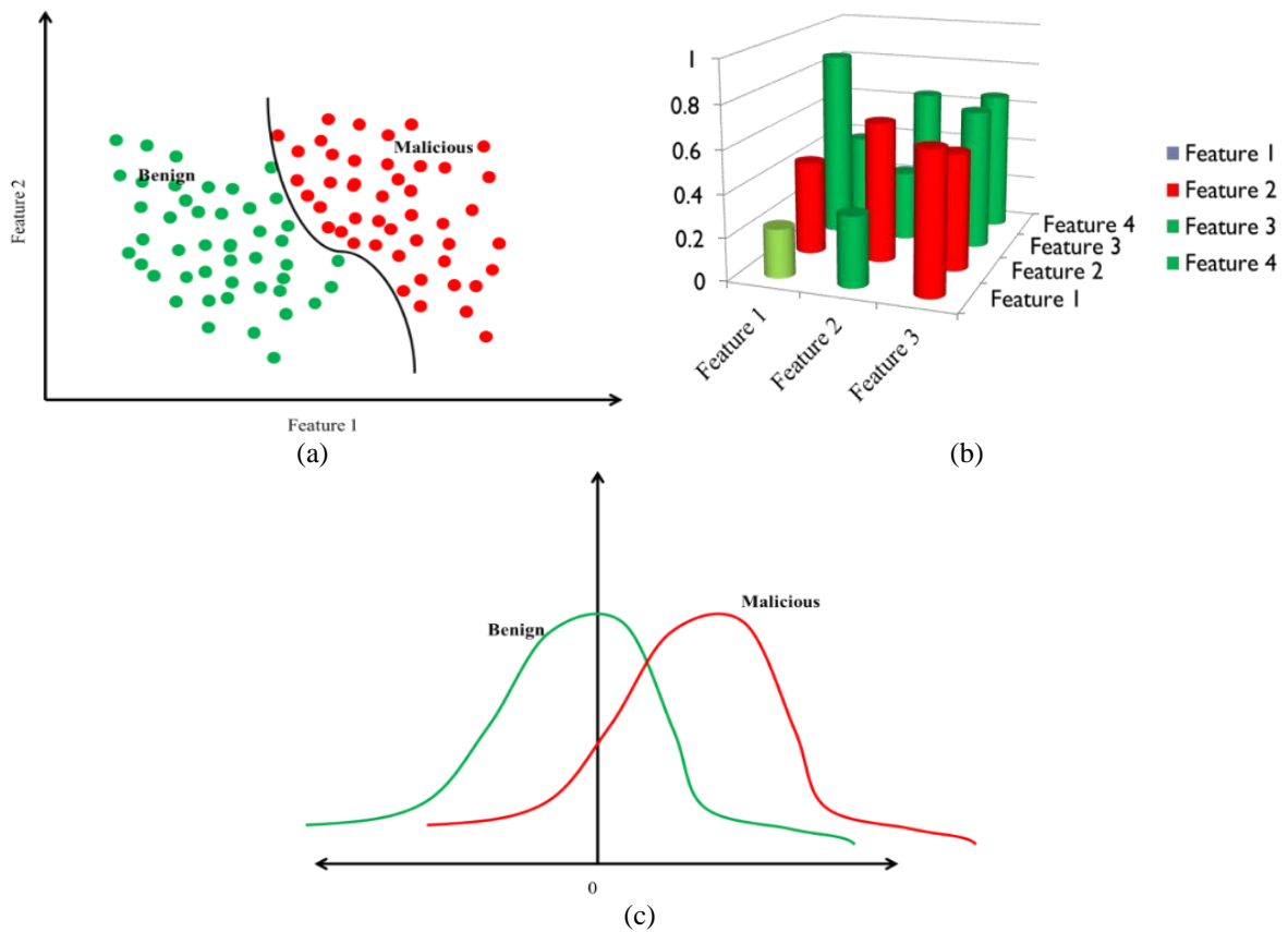
Figure 4. Naïve Bayes classifier model (a) Gaussian, (b) Multinomial, and (c) Bernoulli
