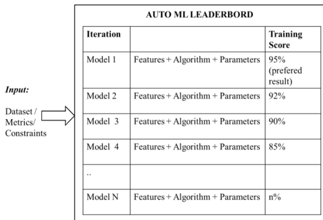
Figure 2. AutoML model
