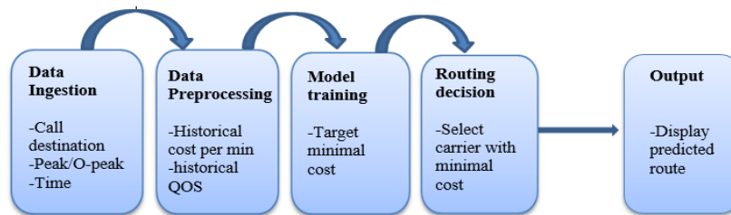
Figure 3. Overall workflow of the optimal route prediction model
