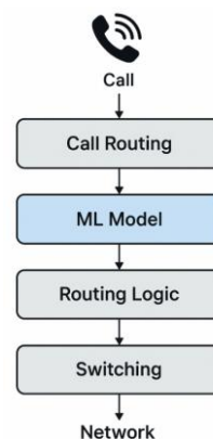
Figure 1. ML model integration within the telecom call routing stack
