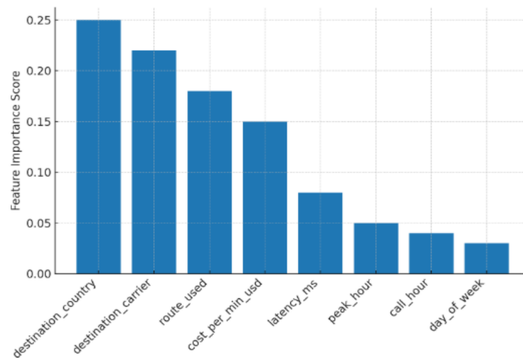
Figure 2. Random forest feature importance for least-cost routing
