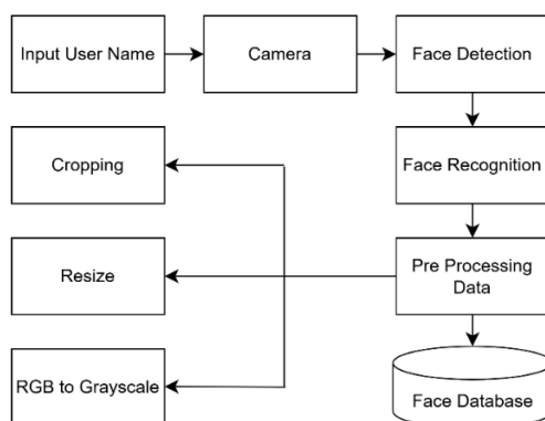
Figure 1. Dataset creation flow
