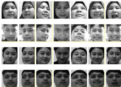
Figure 3. Image dataset
