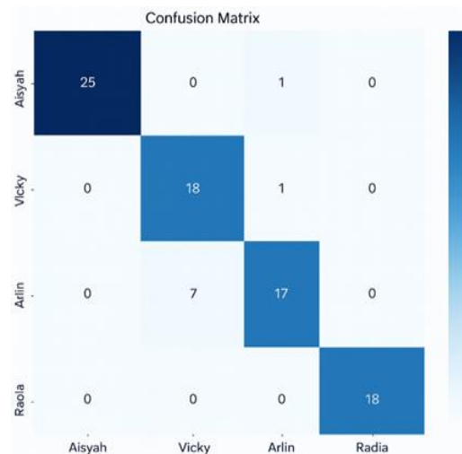
Figure 7. Heatmap confusion matrix
