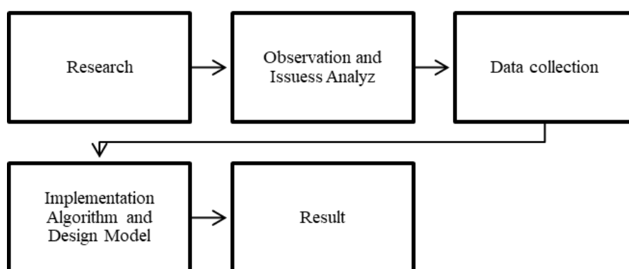
Figure 3. Research flow
