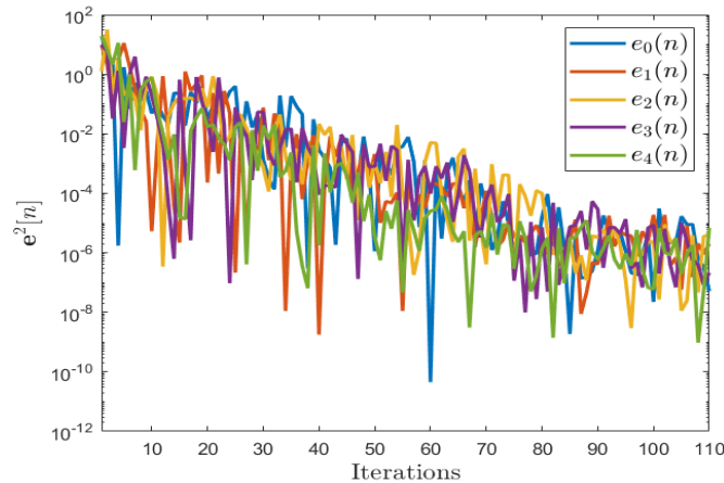
Figure 3. Squared NLMS-error term e[n] in (14) showing algorithm convergence properties
