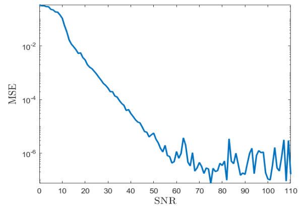
Figure 5. Element-wise MSE between W and H^{-1} , computed for a range of SNR values
