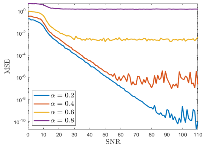
Figure 6. Element-wise MSE between W and H^{-1} , computed for a range of matrix conditions
