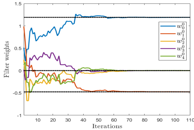
Figure 2. Filter weights w^i[n] in (13) with i = 0 , depicting first-row estimates of inverse matrix W
