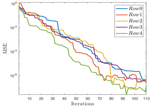
Figure 4. Element-wise MSE between respective rows of W and H^{-1}
