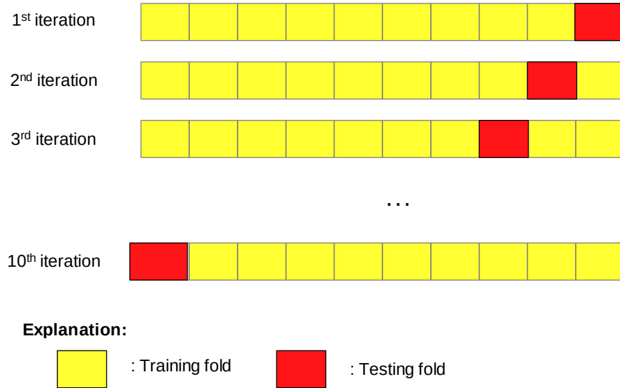
Figure 3. K-Fold cross validation with k=10
