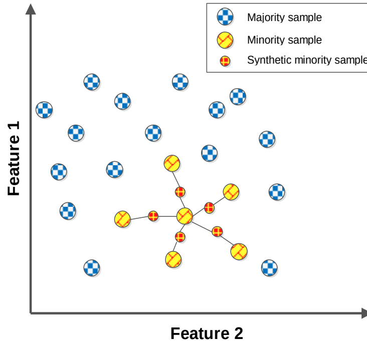
Figure 2. SMOTE illustration
