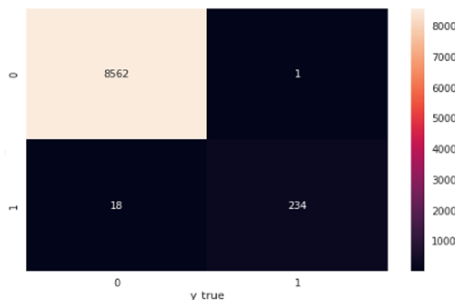
Figure 10. Confusion matrix display
