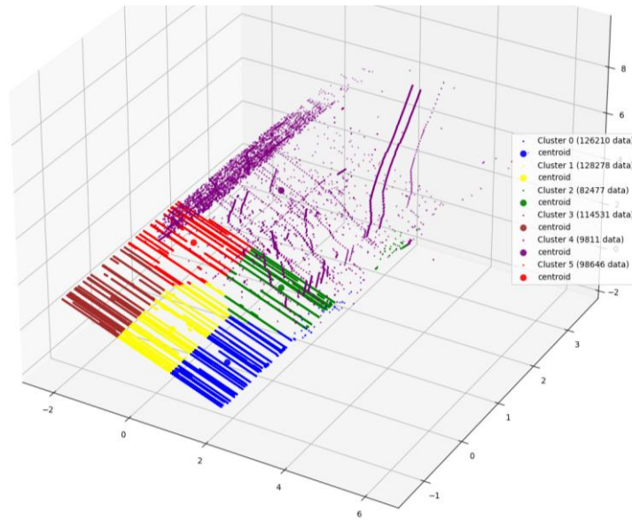
Figure 7. Clustering result
